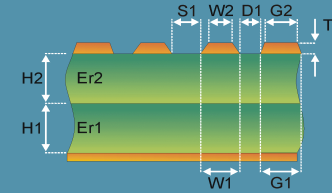
Diff Surface Coplanar Strips With Ground 2B
