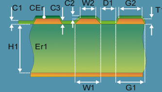
Coated Coplanar Strips With Ground 1B
