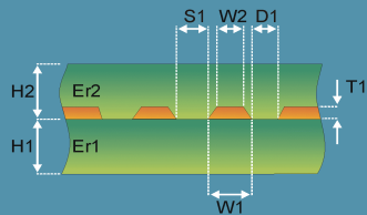
Diff Embedded Coplanar Waveguide 1B1A
