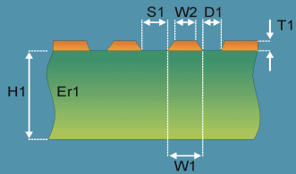
Diff Surface Coplanar Waveguide 1B
