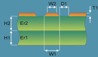
Surface Coplanar Waveguide 2B
