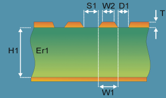
Diff Surface Coplanar Waveguide With Ground 1B
