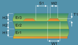
Edge-Coupled Embedded Microstrip 2B1A
