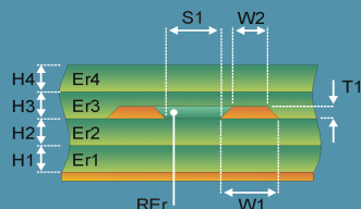
Edge-Coupled Embedded Microstrip 2B2A1R
