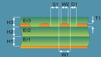
Diff Embedded Coplanar Waveguide With Ground 2B1A
