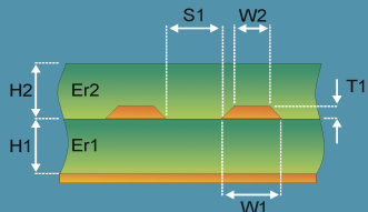
Edge-Coupled Embedded Microstrip 1B1A
