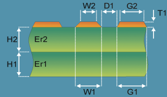
Surface Coplanar Strips 2B
