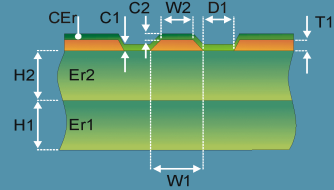
Coated Coplanar Waveguide 2B
