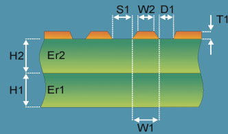
Diff Surface Coplanar Waveguide 2B
