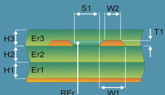
Edge-Coupled Embedded Microstrip 2B1A1R
