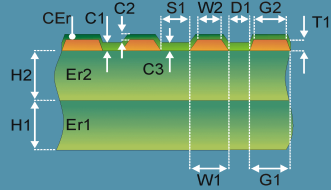
Diff Coated Coplanar Strips 2B
