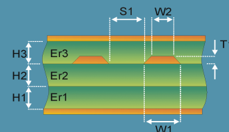
Edge-Coupled Offset Stripline 2B1A
