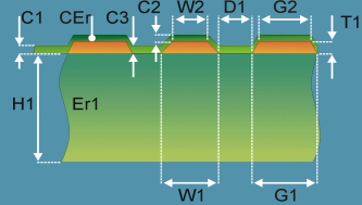
Coated Coplanar Strips 1B
