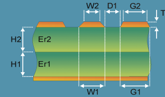
Surface Coplanar Strips With Ground 2B
