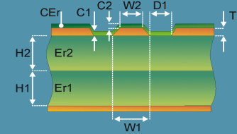
Coated Coplanar Waveguide With Ground 2B
