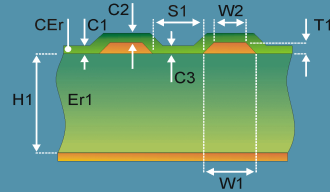
Edge-Coupled Coated Microstrip 1B
