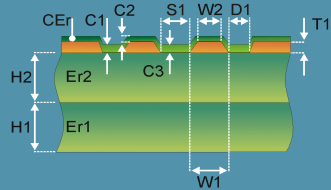
Diff Coated Coplanar Waveguide 2B
