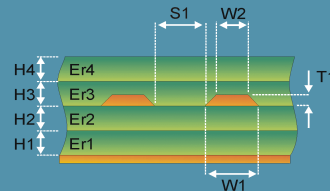
Edge-Coupled Embedded Microstrip 2B2A
