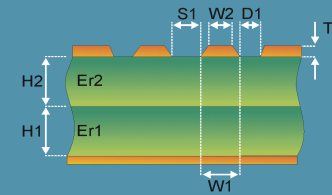
Diff Surface Coplanar Waveguide With Ground 2B
