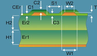
Edge-Coupled Coated Microstrip 2B
