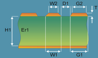
Surface Coplanar Strips With Ground 1B
