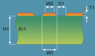
Surface Coplanar Waveguide 1B
