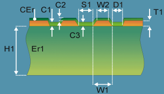
Diff Coated Coplanar Waveguide 1B
