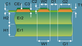
Coated Coplanar Strips 2B
