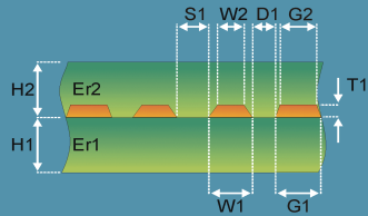
Diff Embedded Coplanar Strips 1B1A
