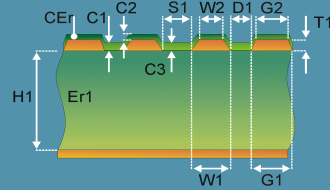
Diff Coated Coplanar Strips With Ground 1B
