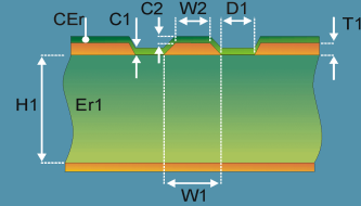
Coated Coplanar Waveguide With Ground 1B
