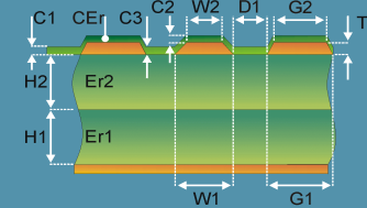
Coated Coplanar Strips With Ground 2B
