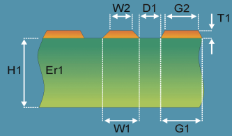
Surface Coplanar Strips 1B
