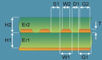
Diff Embedded Coplanar Strips With Ground 1B1A
