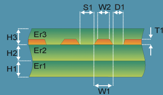
Diff Embedded Coplanar Waveguide 2B1A
