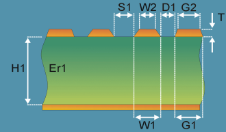
Diff Surface Coplanar Strips With Ground 1B
