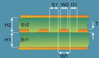
Diff Offset Coplanar Waveguide 1B1A
