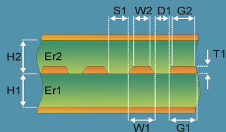
Diff Offset Coplanar Strips 1B1A
