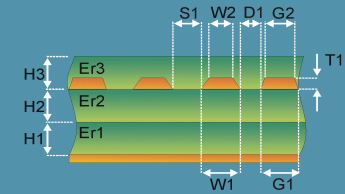
Diff Embedded Coplanar Strips With Ground 2B1A
