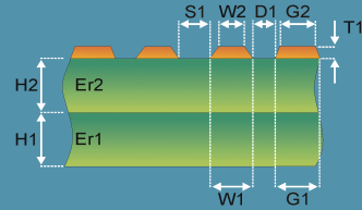
Diff Surface Coplanar Strips 2B
