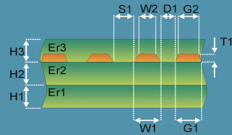
Diff Embedded Coplanar Strips 2B1A
