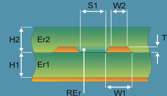
Edge-Coupled Embedded Microstrip 1B1A1R
