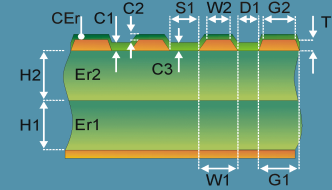
Diff Coated Coplanar Strips With Ground 2B
