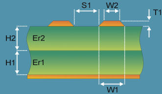
Edge-Coupled Surface Microstrip 2B
