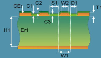
Diff Coated Coplanar Waveguide With Ground 1B
