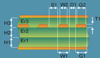
Diff Offset Coplanar Strips 2B1A
