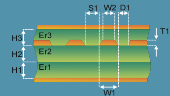
Diff Offset Coplanar Waveguide 2B1A
