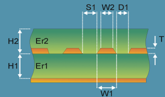
Diff Embedded Coplanar Waveguide With Ground 1B1A
