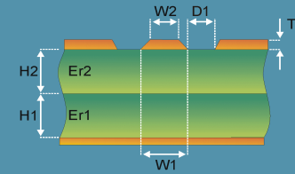
Surface Coplanar Waveguide With Ground 2B
