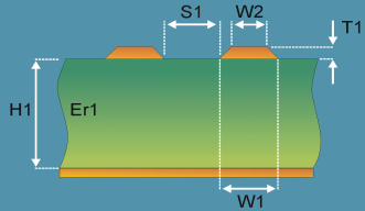
Edge-Coupled Surface Microstrip 1B
