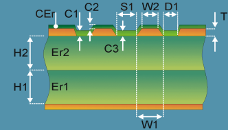
Diff Coated Coplanar Waveguide With Ground 2B
