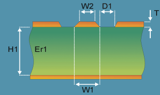
Surface Coplanar Waveguide With Ground 1B
