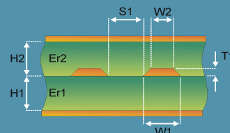
Edge-Coupled Offset Stripline 1B1A
