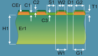
Diff Coated Coplanar Strips 1B
