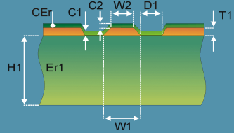
Coated Coplanar Waveguide 1B
