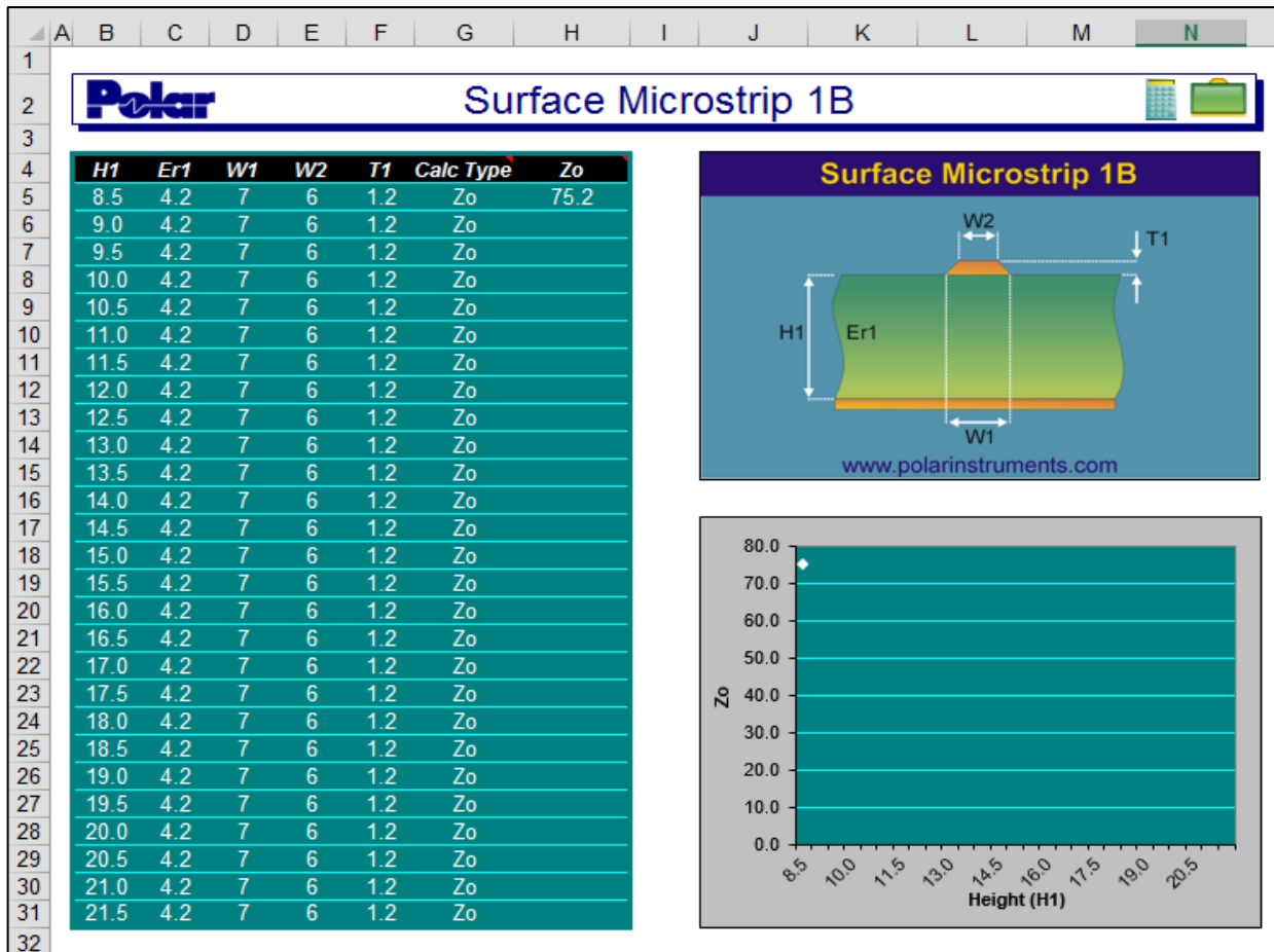
Surface Microstrip sample worksheet
