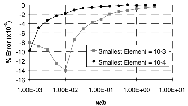
Figure 5 - Substrate \epsilon_r = 4.2
