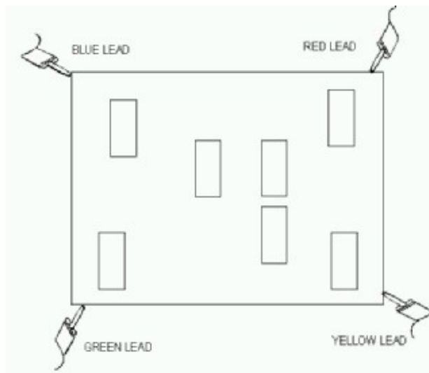
VPS connections to a plane
